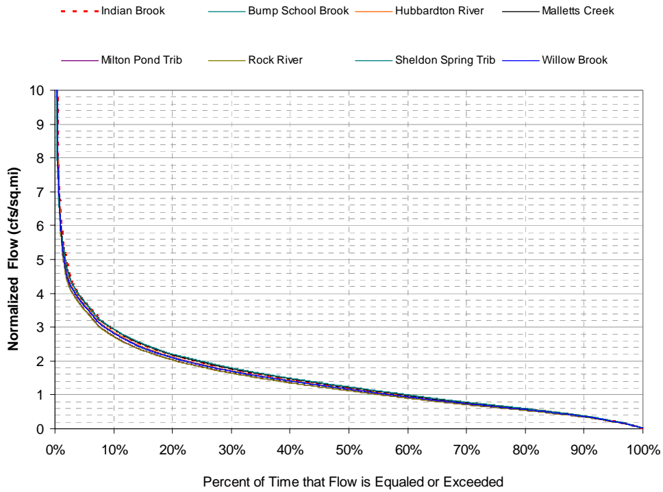
Figure 4. Flow duration curves for Indian Brook and attainment streams.
