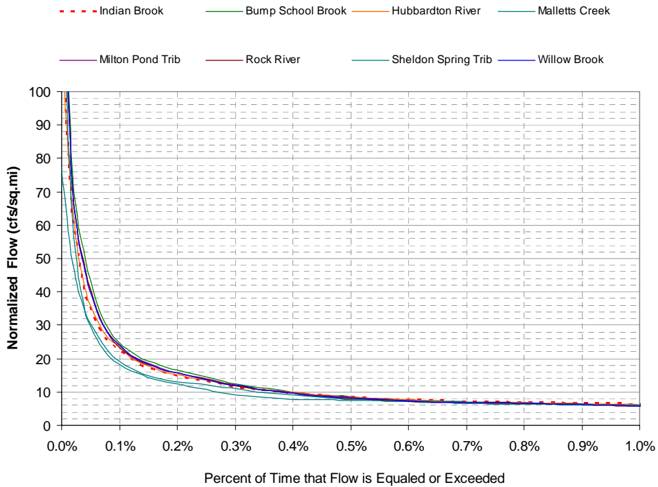
Figure 5. High flow portion of the flow duration curves for Indian Brook and attainment streams
