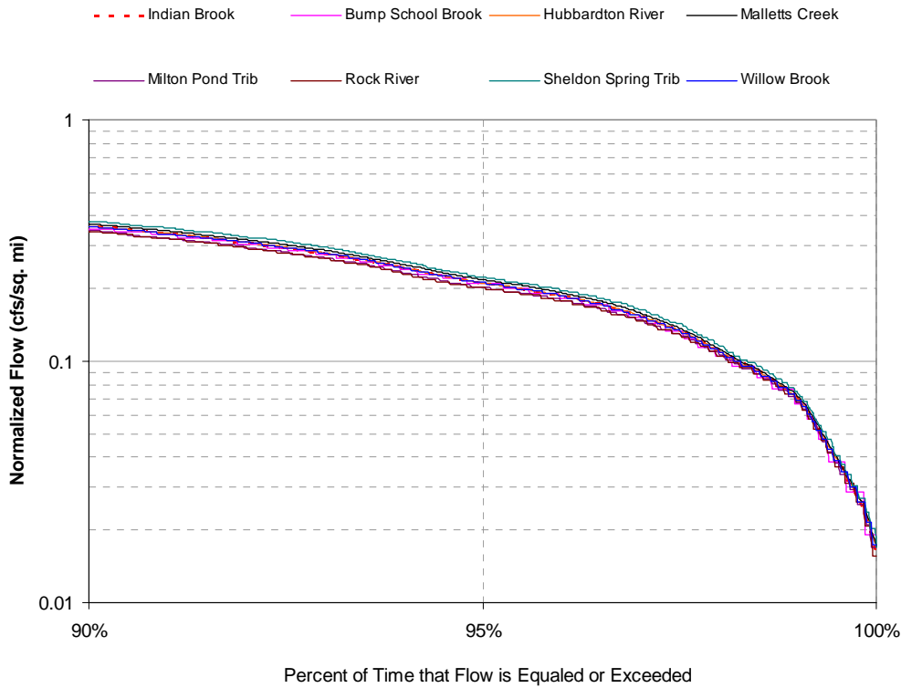
Figure 6. Low flow portion of the flow duration curves for Indian Brook and attainment streams.
